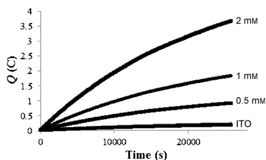
Figure 3. Chronocoulometric ( Q = charge vs. time) plot from controlled-potential electrolysis with \text{Cu}^{\text{II}}(\text{Py}_3\text{P}) ( [\text{1}] = 2 mM, 1 mM, and 0.5 mM) at a tin-doped indium oxide working electrode (ITO, 0.7 \text{cm}^2 ) and pH 8.0 (0.1 M phosphate, \mu = 0.5 M with added \text{LiClO}_4 ) at an applied potential of 1.4 V versus NHE. A charge-versus-time trace for the background ITO electrode is also shown.
