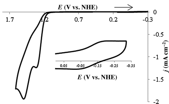
Figure 2. Cyclic voltammogram of \text{Cu}^{\text{II}}(\text{Py}_3\text{P}) ( 1 , 0.7 mM) at pH 8.0 (0.1 M phosphate buffer, \mu = 0.5 M) at a boron-doped diamond working electrode (BDD, 0.07 \text{cm}^2 , 100 \text{mV s}^{-1} , 293 K) with the arrow indicating the initial scan direction. The inset shows a magnified view of the \text{Cu}^{\text{II/I}} wave at -0.14 V versus NHE.
