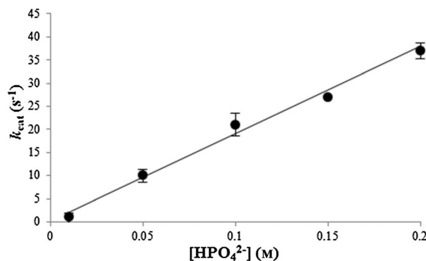
Figure 5. Plot of the catalytic rate constant ( k_{\text{cat}} ) versus [\text{HPO}_4^{2-}] ( \text{M} ) for water oxidation by \text{Cu}^{\text{II}}(\text{Py}_3\text{P}) ( 1 ) at pH 8.0 ( \mu = 0.5 \text{ M} with added \text{LiClO}_4 ) at room temperature.
